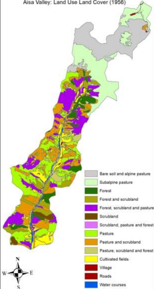
Aisa Valley: Land Use Land Cover (1956)
