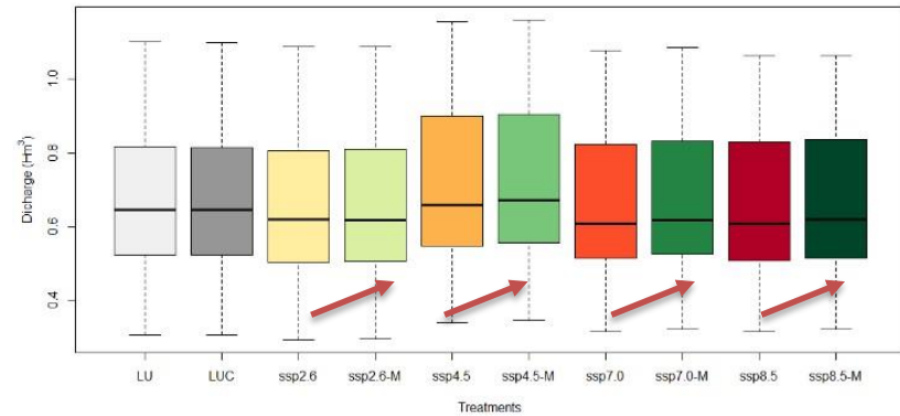
Annual Discharge - Aisa (2070-2099)
