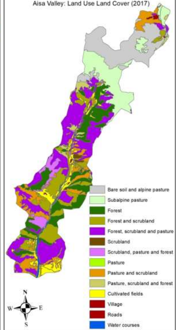
Aisa Valley: Land Use Land Cover (2017)
