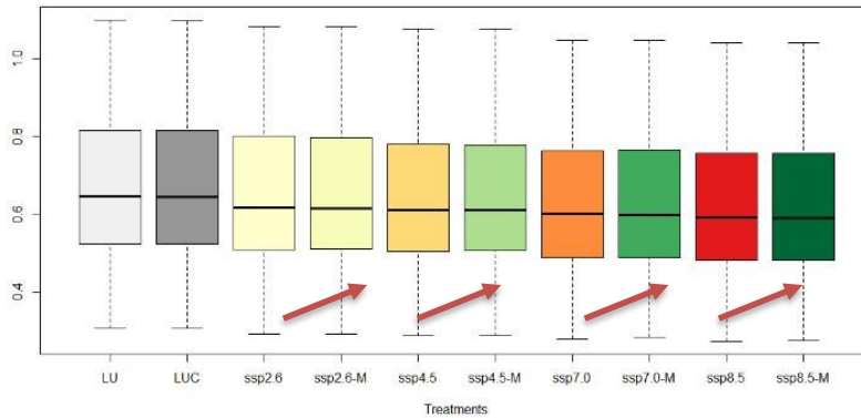
Annual Discharge - Aisa (2035-2064)
