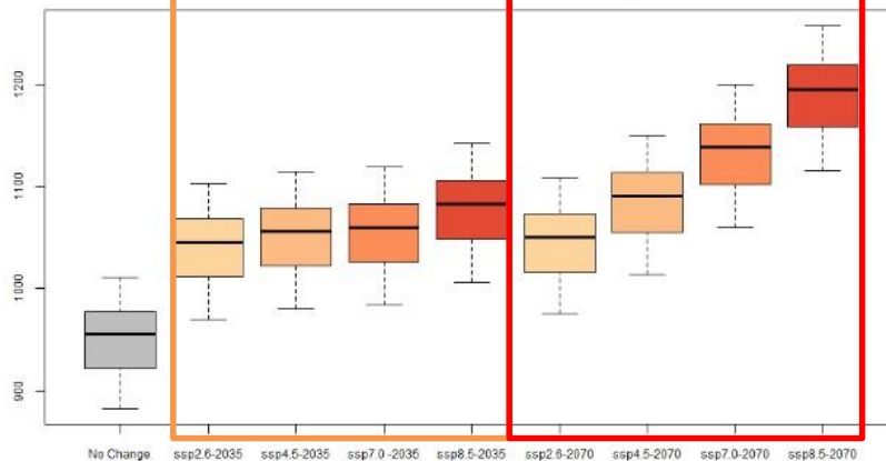
Atmospheric Evaporative Demand [Hargreaves](mm) - Aisa
