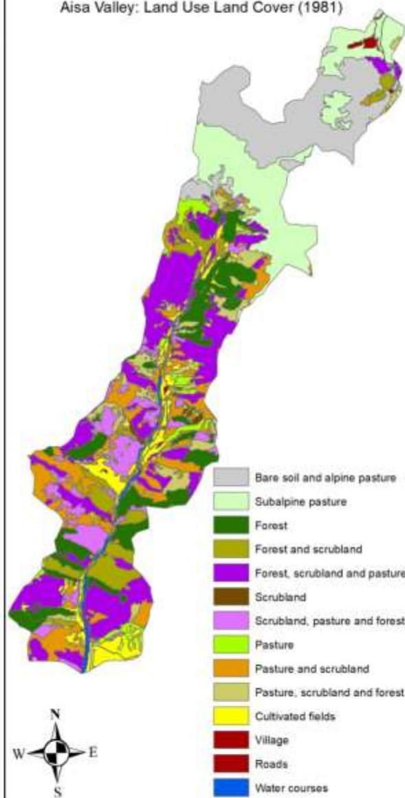
Aisa Valley: Land Use Land Cover (1981)
